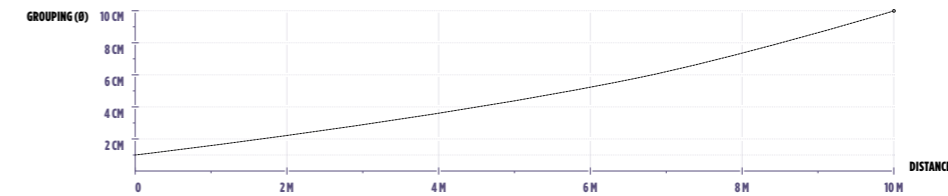
ACCURACY — 10 CM GROUPING (Ø) AT A DISTANCE OF 10 METERS SHOT WITH T4E FASTBALLS, CAL. 43 (ITEM NO. 2.4771-1), 10 ROUNDS
