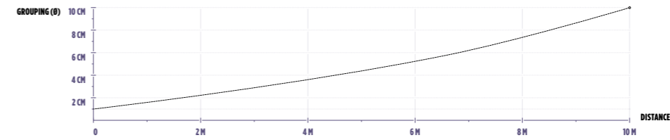
ACCURACY — 10 CM GROUPING (Ø) AT A DISTANCE OF 10 METERS SHOT WITH T4E FASTBALLS, CAL. 43 (ITEM NO. 2.4771-1), 10 ROUNDS
