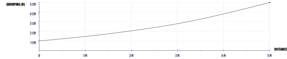
ACCURACY — 5 CM GROUPING (Ø) AT A DISTANCE OF 5 METERS SHOT WITH T4E FASTBALLS, CAL. 43 (ITEM NO. 2.4771-1), 8 ROUNDS
