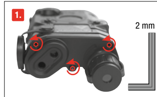
Loosen screws
